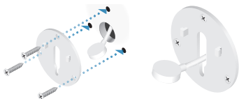
Securing the Instant PoE Wall Mount
